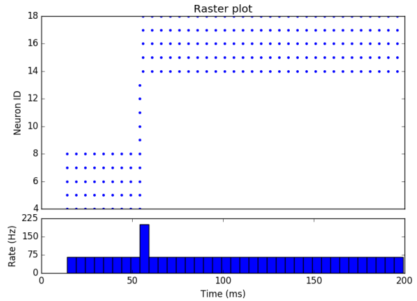
Fig. 3. Raster plot for the simulated neurons. Firing of five neurons occurs after 15ms and the next neuron population fires after 50ms. The persistent responses of two neuron populations are shown here.
